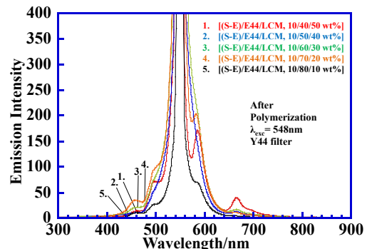
Fig.4 Fluorescence spectra of [(S-E)/E44/LCM] composite films with photon upconversion dyes system after photopolymerization in air.
