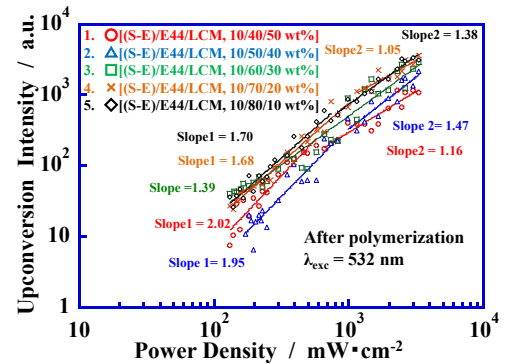
Fig.8 Excitation light intensity dependence of photon UC fluorescence of [(S-E)/E44/LCM] photon UC dyes composite films after photopolymerization in air at \lambda_{exc} = 532 nm.
